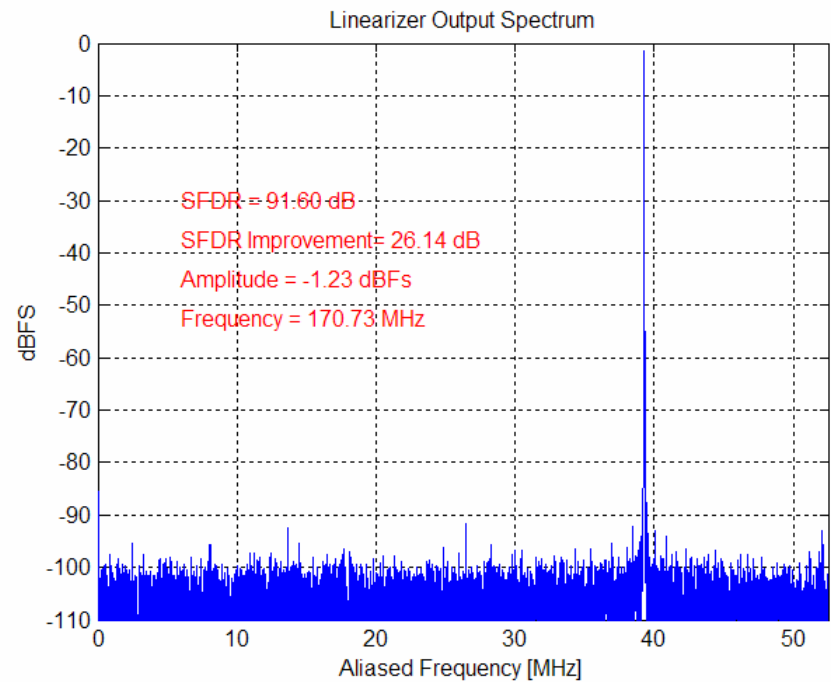
Linearized Output
